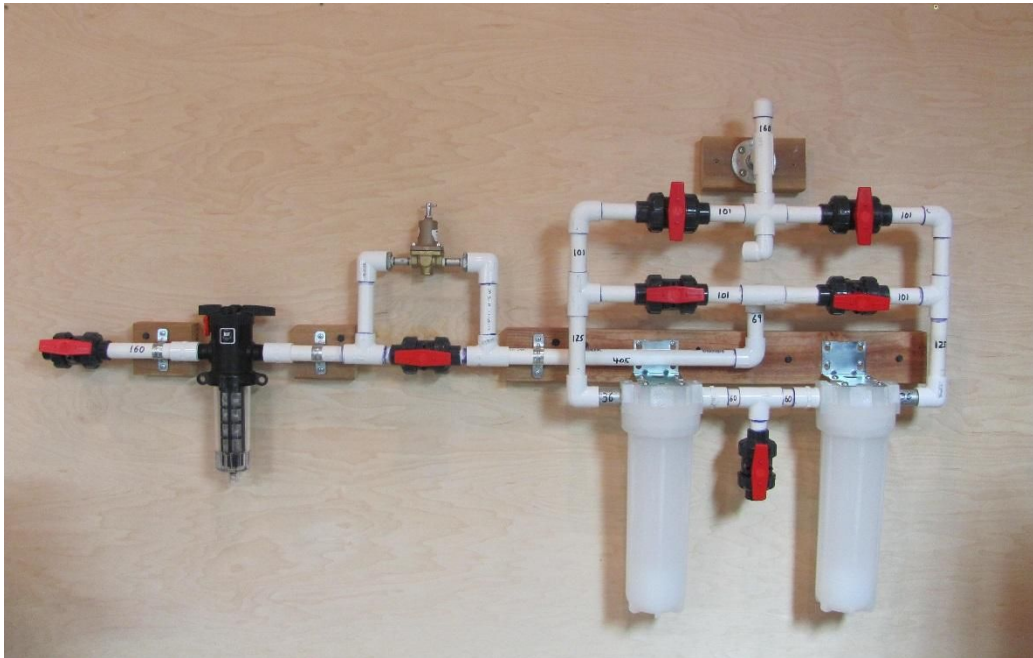
NORMAL OPERATING POSITION
