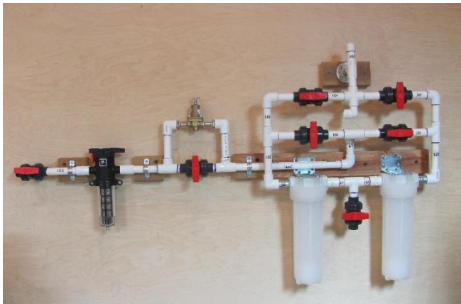
BACKFLUSH LEFT FILTER POSITION
